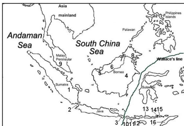
2 The localities of the specimens of M. muricola that were examined. The west of Wallace's Line region is represented by (1) Jambi (2) Krakatau Island (3) Bali Island (4) East Kalimantan (5) Southern Sarawak (6) Central Sarawak (7) Northern Sarawak (8) Tawau, Sabah (9) Fraser Hill, Pahang. The sites from the east of Wallace's Line include: (10) Lombok Island (11) Sumbawa Island (12) Sumba Island (13) Flores Island (14) Lembata Island (15) Pantar Island (16) Timor Island
